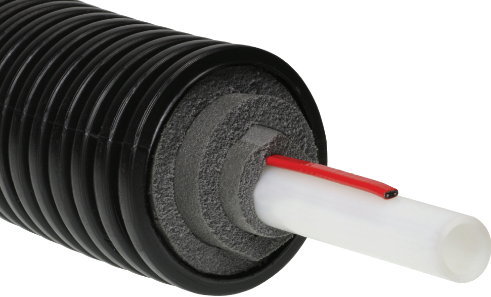
5455513 1¼" Potable PEX Plus with 5.5" Jacket, 7 W/ft.
