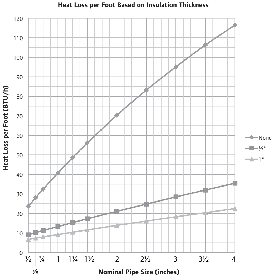
Figure 15-1: Distribution Pipe Heat Loss per Foot
