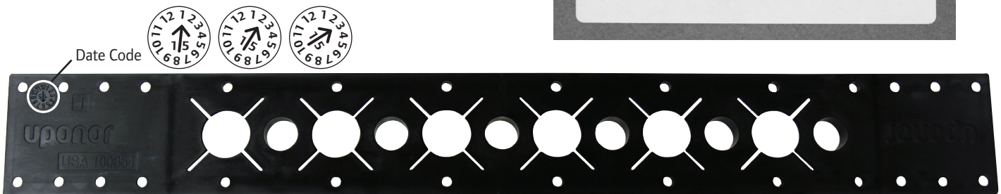
PEX Wall Support Bracket, ½" and ¾" (A5750500)
